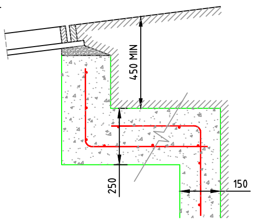
HAUNCHED DETAIL
