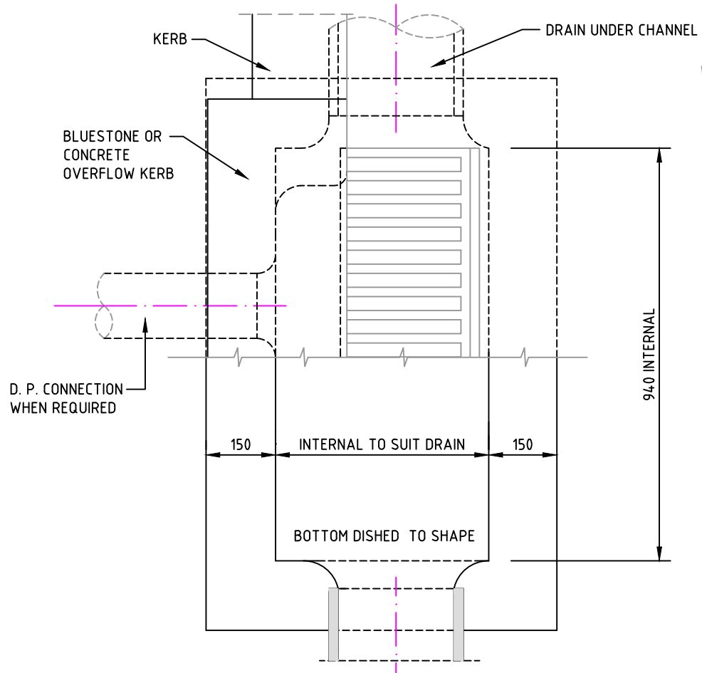
PLAN AND SECTION
