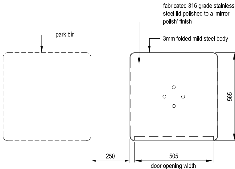
Section
