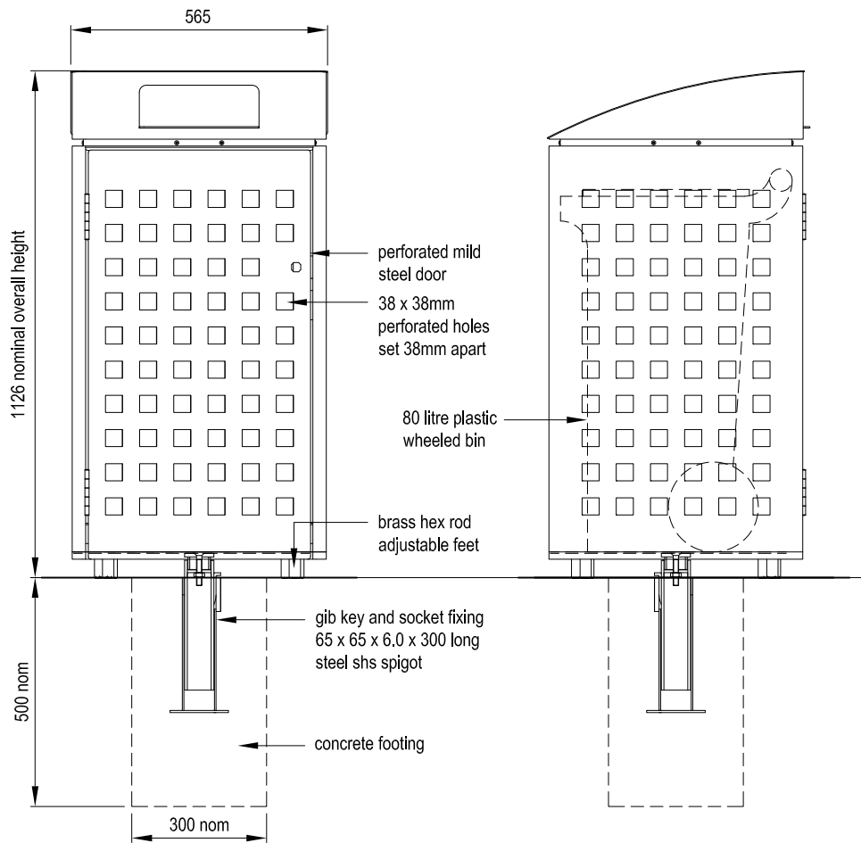
Section / Elevations
