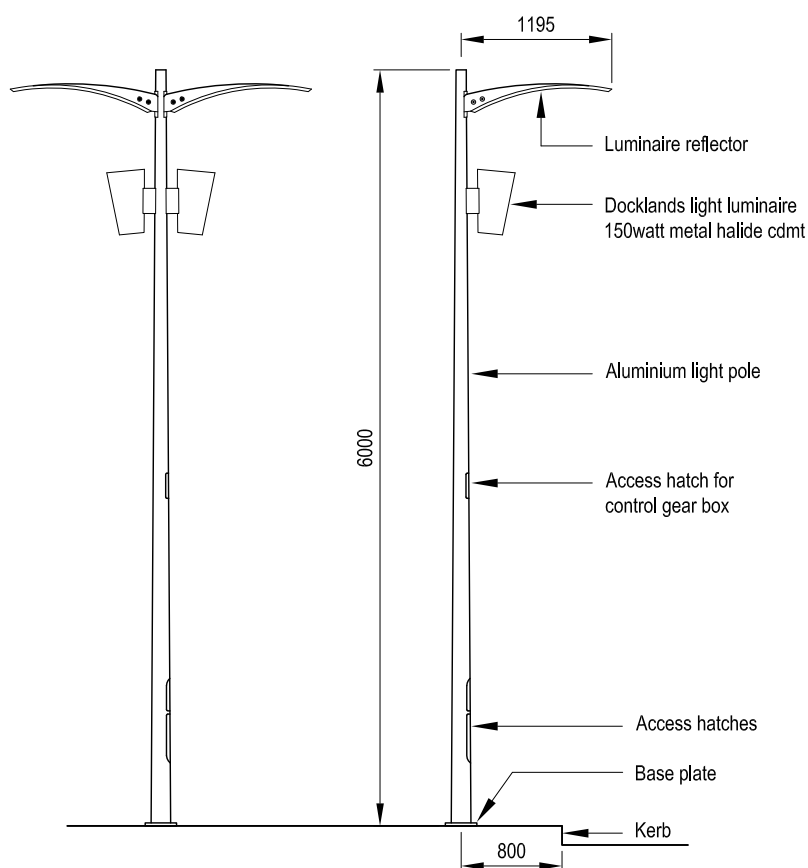
Elevations
