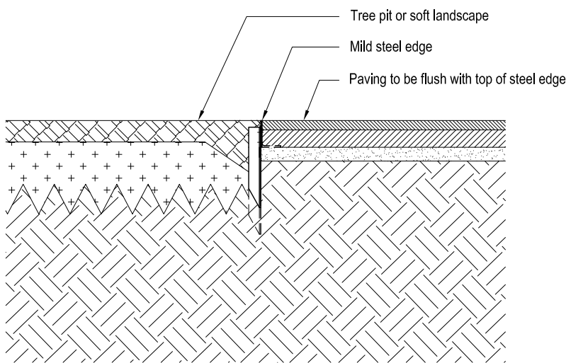
Section: Edge of tree pit and asphalt paving
