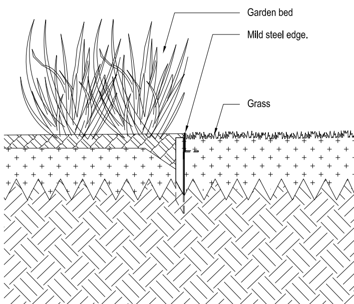
Section: Edge of garden bed and grass
